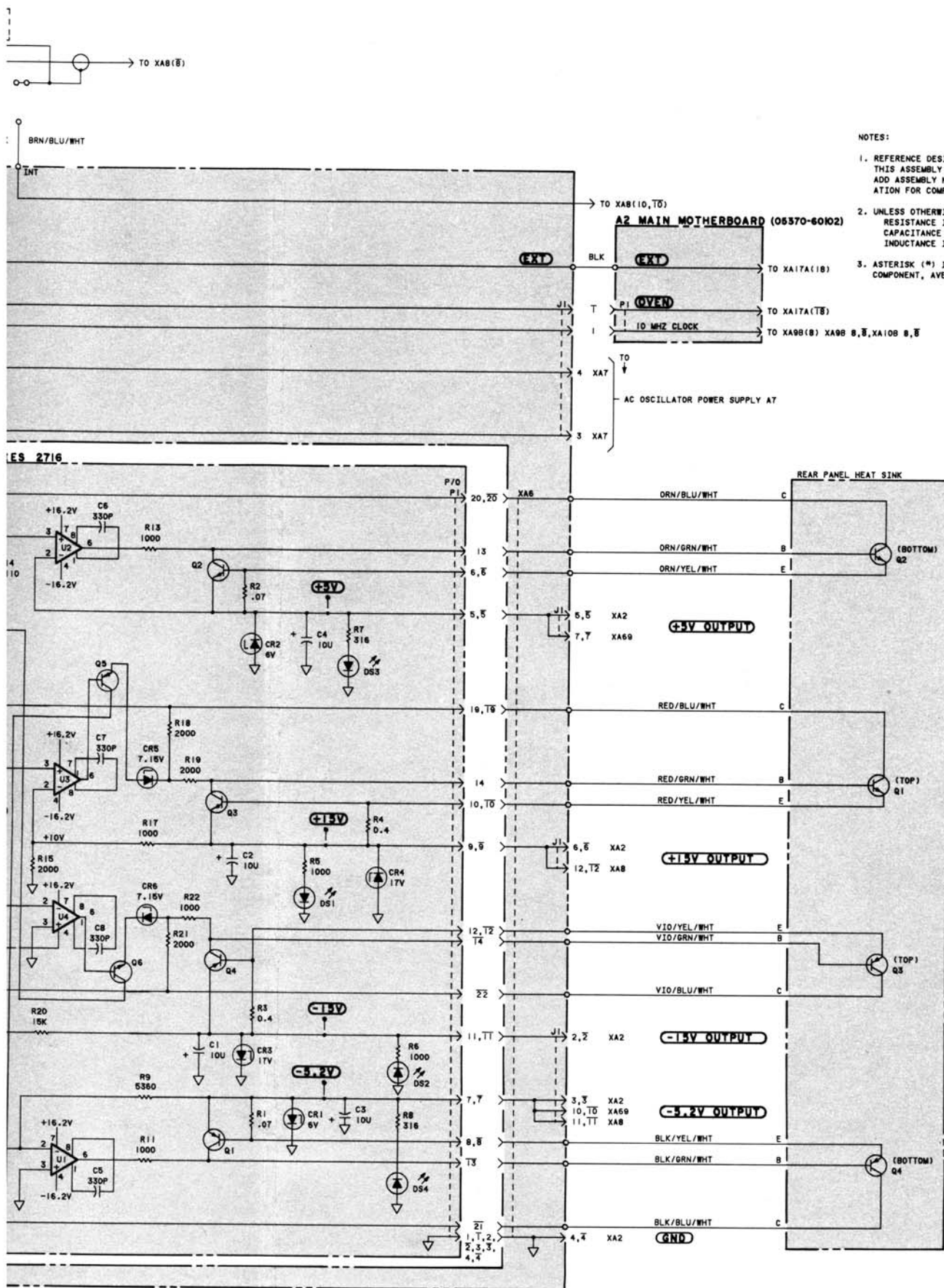
Figure 8-22. A1 Power Supply/Motherboard Assembly, A6 Power Supply Control Assembly A24 Line Module Assembly
